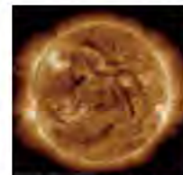
Courtesy of NASA/SDO and the AIA, EVE, and HMI science teams
